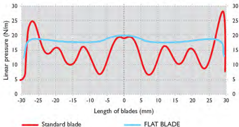
COMPARISON OF AIR PRESSURE DISTRIBUTION BETWEEN A STANDARD BLADE AND A FLAT BLADE.
